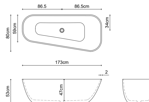
VASCA - BATHTUB ANTBO1
